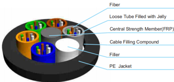
Cable Structure
